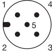
View from soldering side
