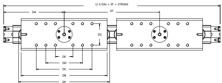
S5 Double Long Carriage Dimensions
