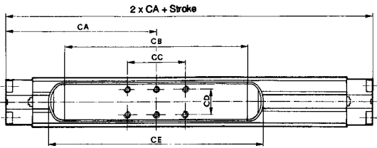
S1 Medium Carriage Dimensions
