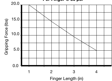
WBG-60 Gripping Force Chart Per Finger @ 80 psi
