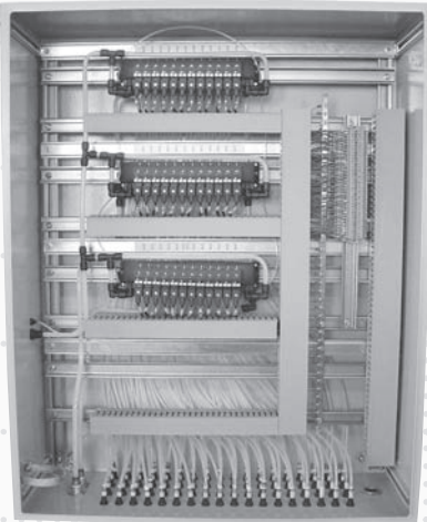
Mega valve islands in cabinet
