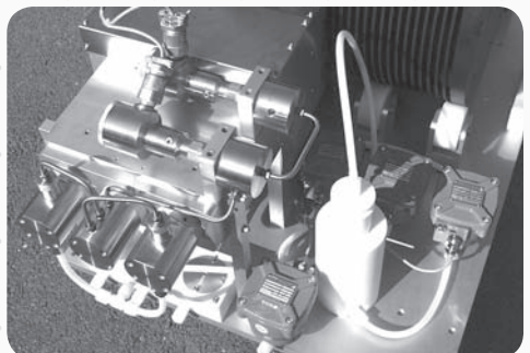
Pumping station for HPLC chromatograph that can be used in explosive areas
